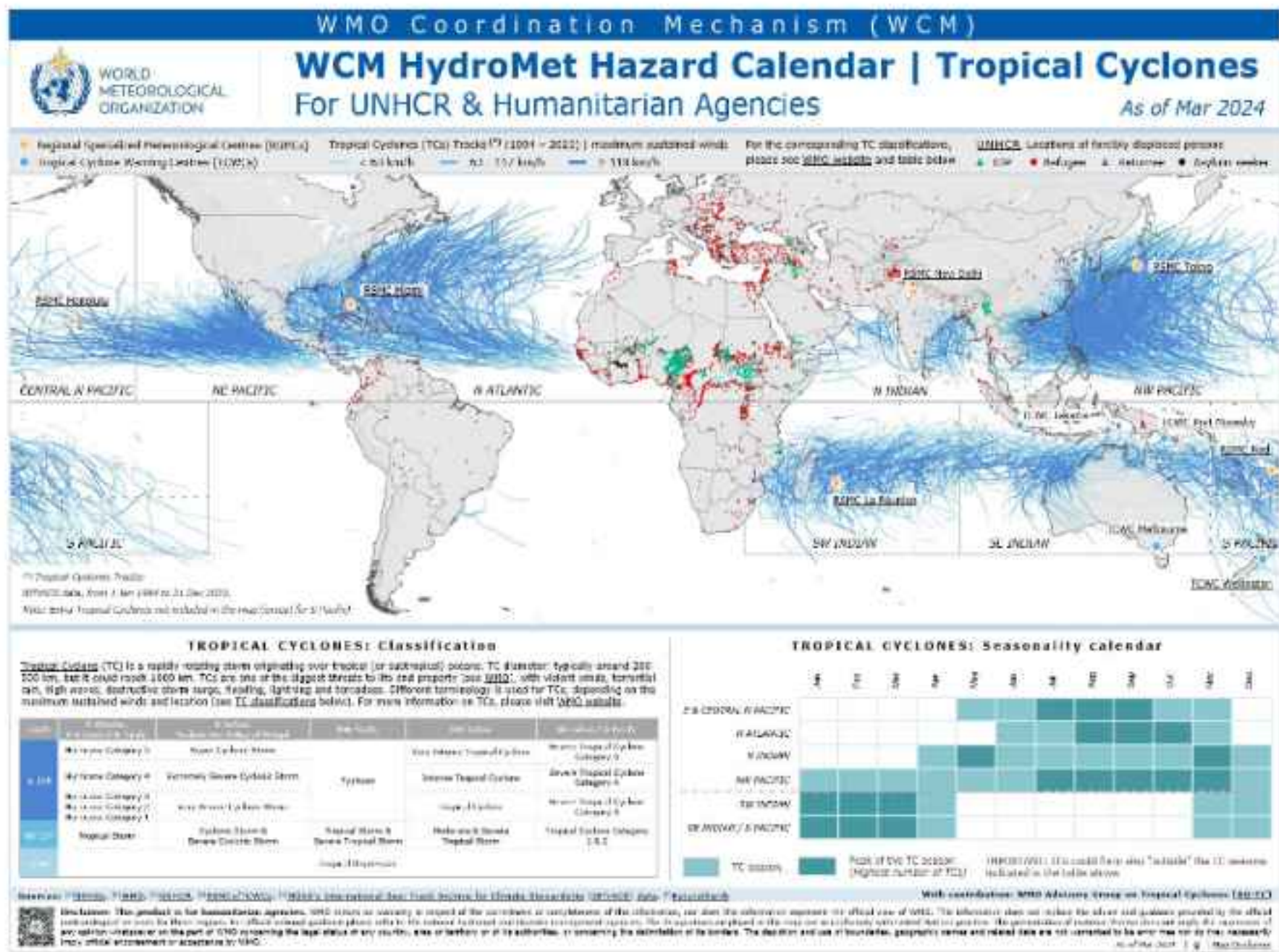
Figure 3.4 WCM Hydromet Hazard Calendar for Tropical Cyclones
